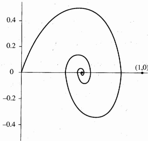
FIGURE 2. THE UNSTABLE MANIFOLD OF THE ORIGIN. ( c = 0.3 ).
