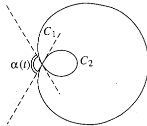
FIGURE 1. A CARDIROIDLIKE CURVE.
